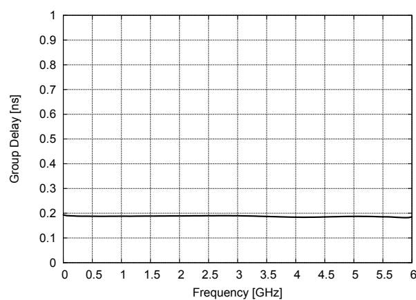
Fig. 4: Group delay between output and input port
