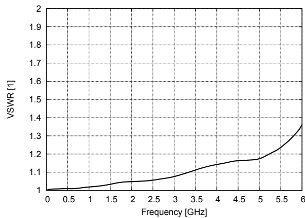
Fig. 2: VSWR for both ports (input and output)
